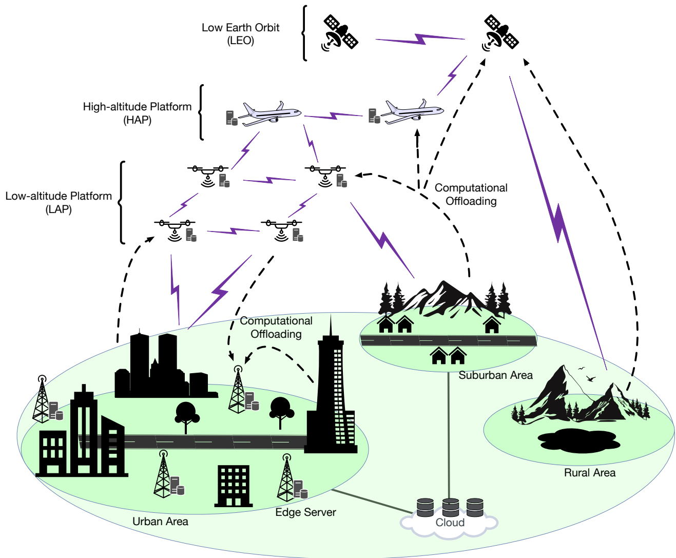
Fig. 1. Air Computing Architecture.
