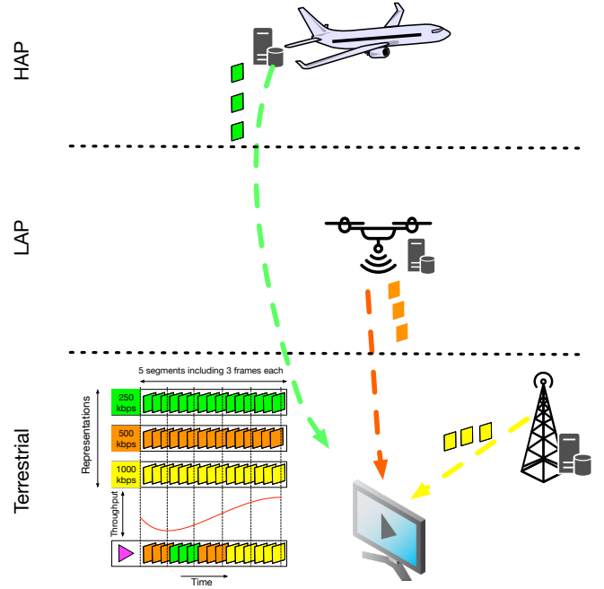
Fig. 7. Different representations of the video segments can be conveyed by different components of air computing based on the network conditions.
